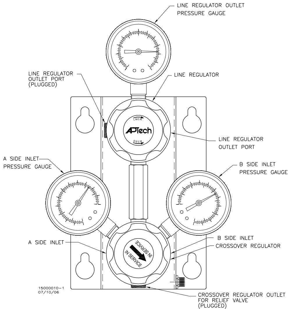
Figure 1. AK M80 Crossover Manifold Front View
