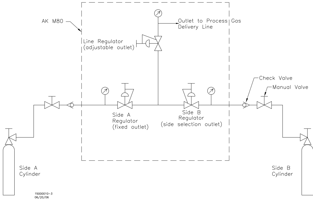
Figure 3. AK M80 Installation Schematic
